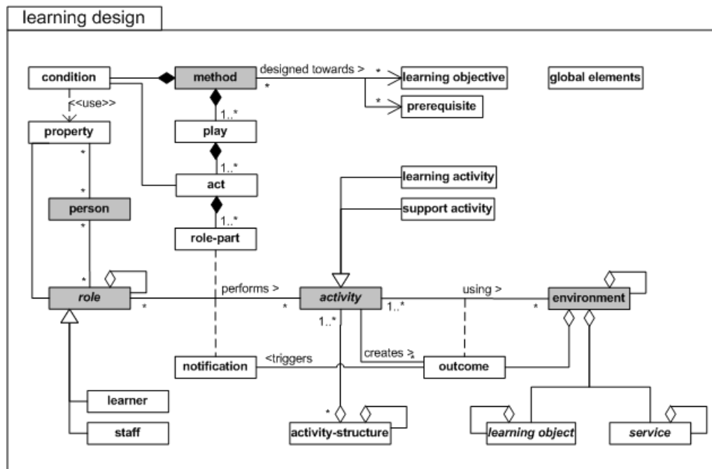
Figure 1: Conceptual structure of the LD specification (Grey colouring is only used to increase the readability).
