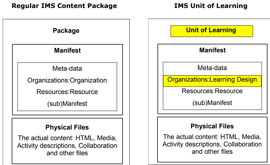
Figure 2. Comparison of a regular IMS CP and an IMS UOL, the UOL is a package where the Organization element is replaced with a Learning Design
